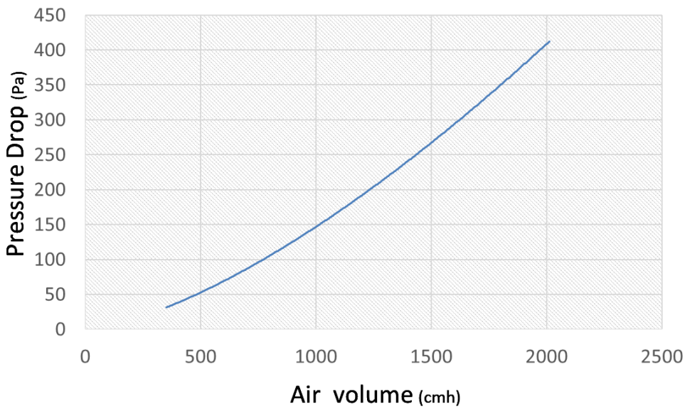
<Pressure drop >
