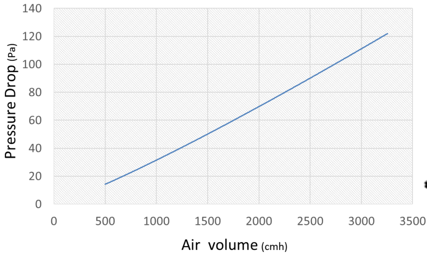
<Pressure drop >
