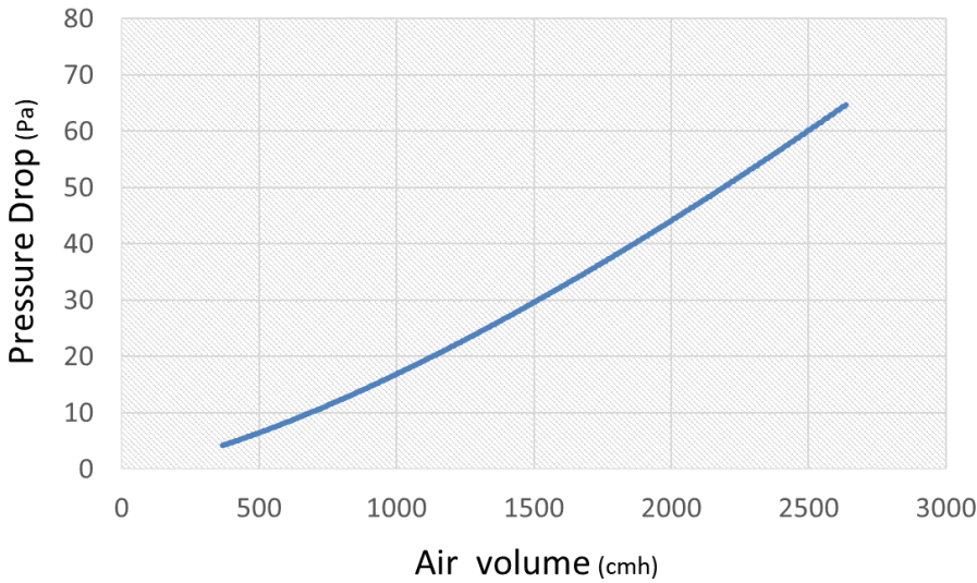
<Pressure drop >
