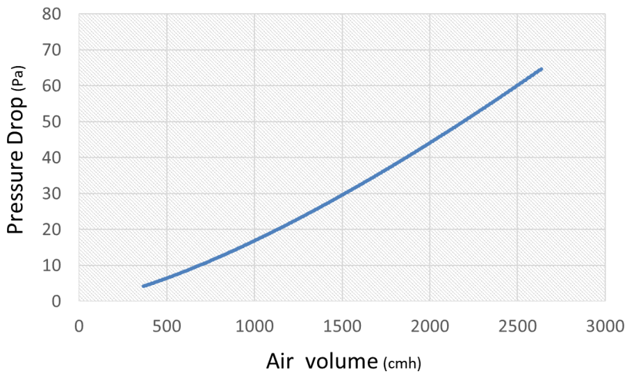
<Pressure drop >
